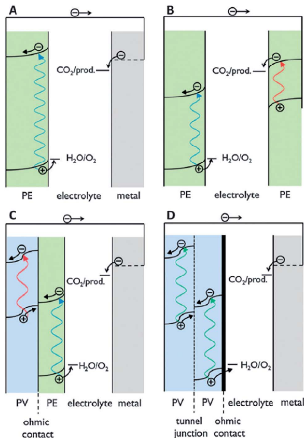
Fig. 2 Four configurations are given for PEC devices for solar fuels evolution in the case of CO 2 reduction. Single semiconductor electrode designs are given in (A) for OER and in (B) for OER and HER at anode and cathode. The corresponding designs featuring buried PV junctions are shown in (C) and (D) (with permission from ref. 30. Copyright 2014 Royal Society of Chemistry).
