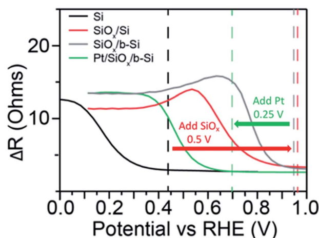
Fig. 5 The thermodynamic flatband potential U_{fb} measured by intensity-modulated high frequency resistivity (IMHFR) spectroscopy at p-type Si electrodes shifts from the bare, hydrogen-terminated Si surface to more positive potentials as an oxide layer is formed at the interface. When Pt catalysts are added to the oxidized Si electrode, the thermodynamic U_{fb} also shifts substantially. (Modified from ref. 76 with permission).
