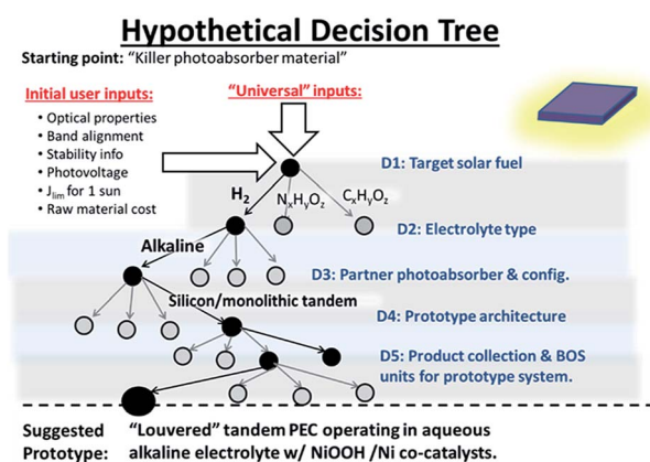
Fig. 3 An example of a decision tree for the design of a PEC device for solar fuels production that starts its flow through decision points "D" with a novel photoabsorbing semiconductor and concludes with a prototype design. Details on the use of this decision tree are given in ESI S2.†
