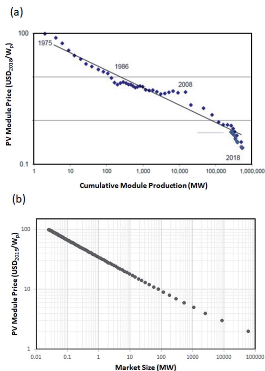
Fig. 1 (a) A learning curve plot using data shows the history of the PV module peak cost ($ per W) with respect to the magnitude of the installed base at that cost (modified from ref. 12). (b) Using the fitted line of (a), the change of the installed base of PV from one year to the next can be plotted as a function of PV module cost for that year in order to show the size of the market for each cost point.
